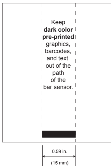
Figure 12 • Label Areas
